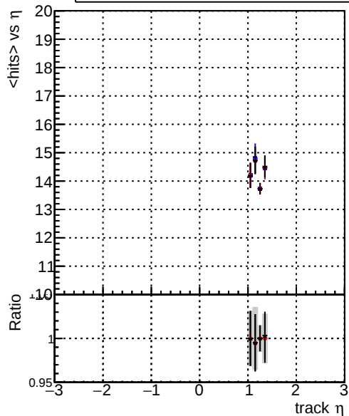
mean hits — DQM_original_step2_pt1to1000_eta1p0to1p4 — DQM_mkFit_step2_pt1to1000_eta1p0to1p4 — DQM_pixelCPETemplate_step2_pt1to1000_eta1p0to1p4
