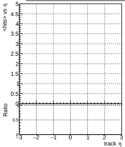
mean hit DQM_original_step2_pt1to1000_eta1p0to1p4 DQM_mkFit_step2_pt1to1000_eta1p0to1p4 DQM_pixelCPETemplate_step2_pt1to1000_eta1p0to1p4
