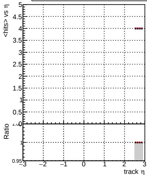
mean hits — DQM_original_step2_pt1000_eta2p5to4p0 — DQM_mkFit_step2_pt1000_eta2p5to4p0 — DQM_pixelCPEtemplate_step2_pt1000_eta2p5to4p0
