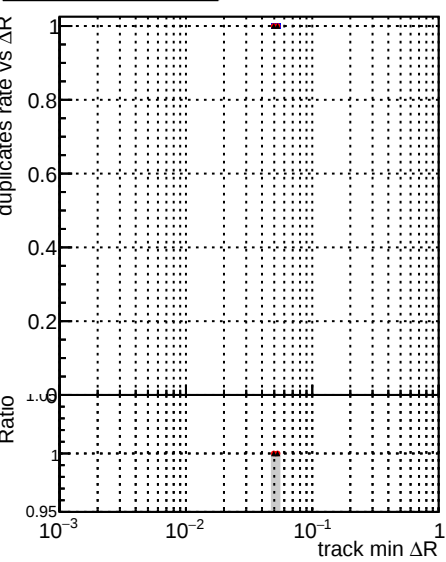
Legend: - blue line with dots: DQM_original_step2_pt1000_eta2p5to4p0 - red line with dots: DQM_mkFit_step2_pt1000_eta2p5to4p0 - black line with dots: DQM_pixelCPETemplate_step2_pt1000_eta2p5to4p0
