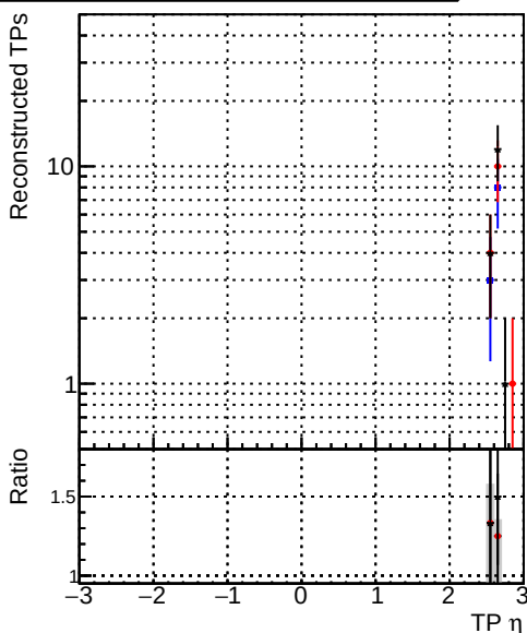
N of simulated tracks vs TP η Legend: DQM_original_step2_pt1000_eta2p5to4p0 DQM_mkFit_step2_pt1000_eta2p5to4p0 DQM_pixelCPETemplate_step2_pt1000_eta2p5to4p0
