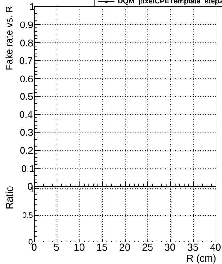
\Lambda tracking fake rate vs R
