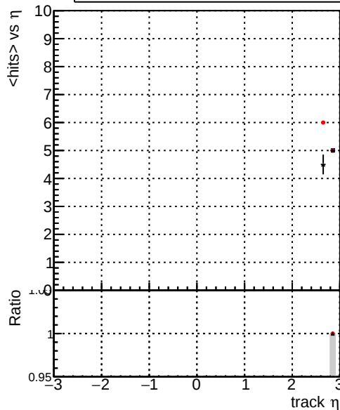
mean hit — DQM_original_step2_pt1000_eta2p5to4p0 — DQM_mkFit_step2_pt1000_eta2p5to4p0 — DQM_pixelCPETemplate_step2_pt1000_eta2p5to4p0
