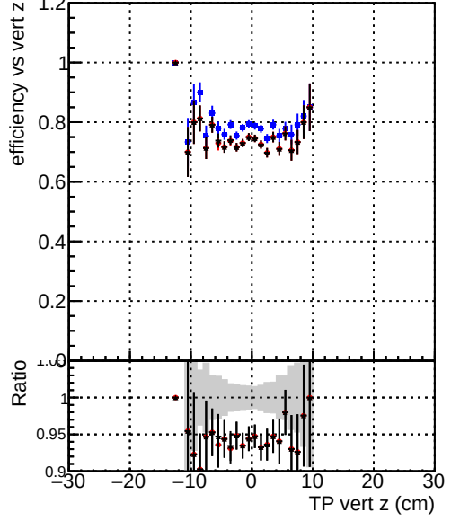
Efficiency vs. Sim. PV z —●— DQM_original_step2_pt1000_eta2p0to2p5 —●— DQM_mkFit_step2_pt1000_eta2p0to2p5 —●— DQM_pixelCPETemplate_step2_pt1000_eta2p0to2p5
