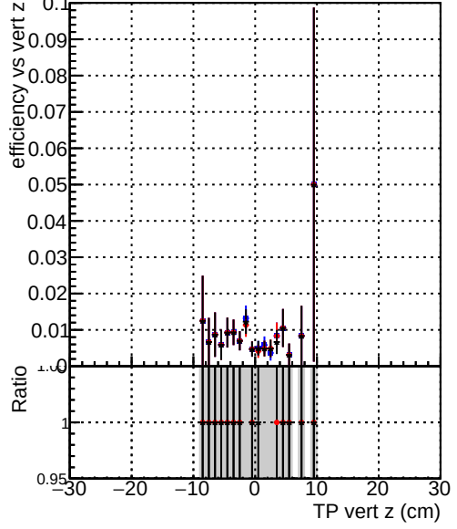
Efficiency vs vert z — DQM_original_step2_pt1000_eta2p0to2p5 — DQM_mkFit_step2_pt1000_eta2p0to2p5 — DQM_pixelCPETemplate_step2_pt1000_eta2p0to2p5
