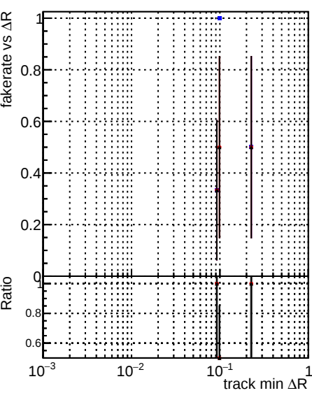
Fake rate vs \Delta R (track, jet) DQM original step2 pt1000 eta2p0to2p5 DQM mkFit step2 pt1000 eta2p0to2p5 DQM pixelCPETemplate step2 pt1000 eta2p0to2p5
