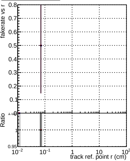
Legend: — DQM original step2_pt1000_eta2p0to2p5 — DQM mkFit step2_pt1000_eta2p0to2p5 — DQM pixelCPETemplate step2_pt1000_eta2p0to2p5
