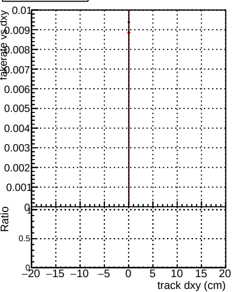
DOM original step2 pt1000 eta2p0to2p5 DOM mkr step2 pt1000 eta2p0to2p5 DOM pixelCPE template step2 pt1000 eta2p0to2p5
