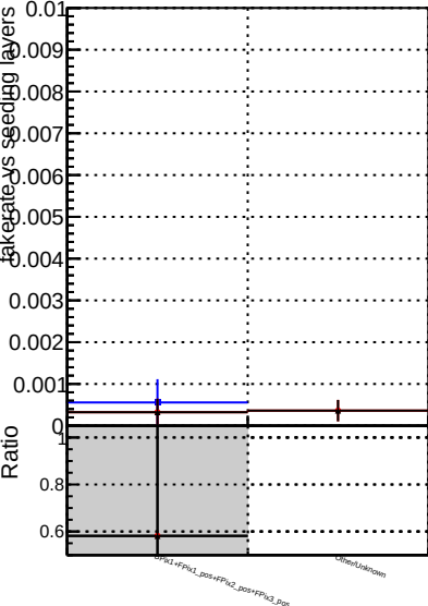
Fake rate vs. DOM original step2 pt1000 eta2p0to2p5 DOM mkr-fit step2 pt1000 eta2p0to2p5 DOM pixelCPE template step2 pt1000 eta2p0to2p5
