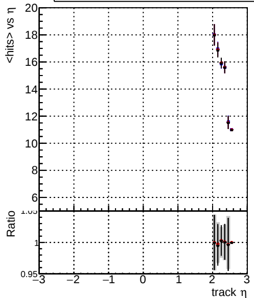
mean hits — DQM_original_step2_pt1000_eta2p0to2p5 — DQM_mkFit_step2_pt1000_eta2p0to2p5 — DQM_pixelCPETemplate_step2_pt1000_eta2p0to2p5
