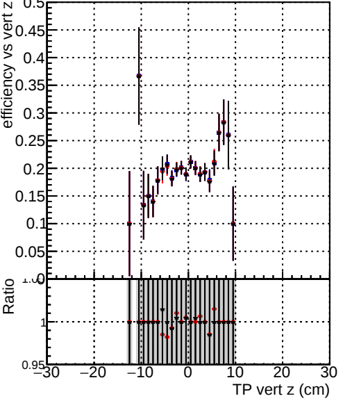
Efficiency vs. sim PV z Legend: DQM_original_step2_pt1000_eta2p0to2p5 DQM_mkFit_step2_pt1000_eta2p0to2p5 DQM_pixelCPETemplate_step2_pt1000_eta2p0to2p5
