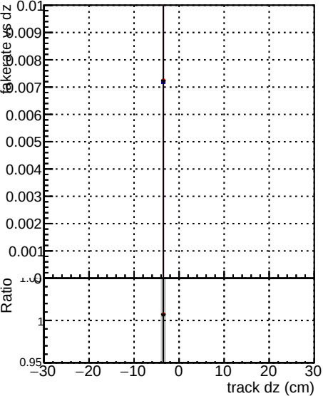
Fake rate vs dz DOM original step2 pt1000 eta2p0to2p5 DOM mkrfit step2 pt1000 eta2p0to2p5 DOM pixelCPE template step2 pt1000 eta2p0to2p5
