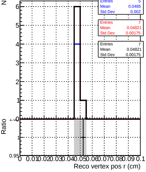
Recons Legend: DQM_original_step2_pt1000_eta1p6to2p0 (blue) DQM_mkFit_step2_pt1000_eta1p6to2p0 (red) DQM_pixelCPETemplate_step2_pt1000_eta1p6to2p0 (black)
