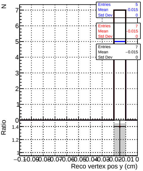
Recons Legend: DQM_original_step2_pt1000_eta1p6to2p0 (blue) DQM_mkFit_step2_pt1000_eta1p6to2p0 (red) DQM_pixelCPETemplate_step2_pt1000_eta1p6to2p0 (black)
