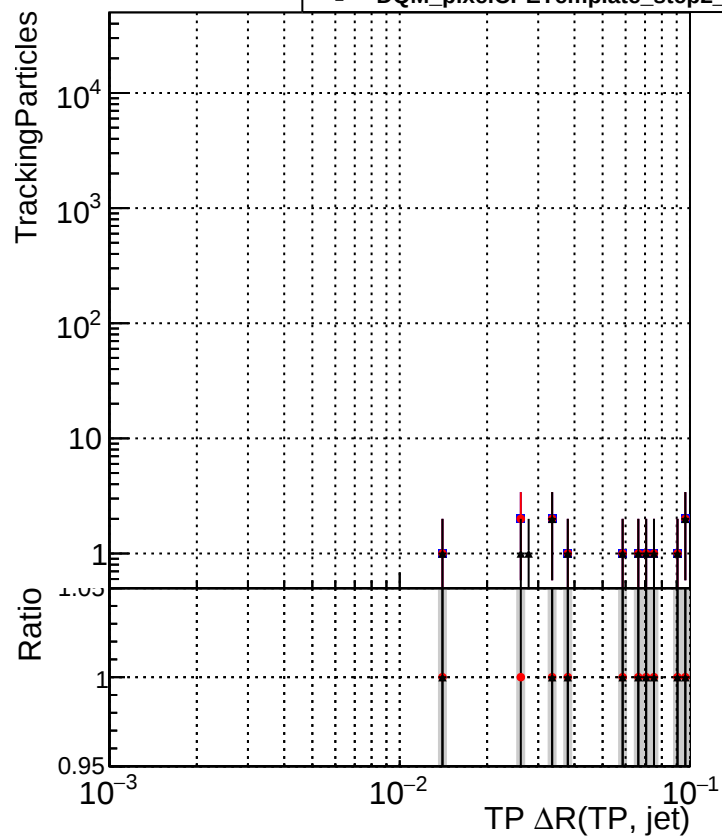
N of simulated tracks vs TP \Delta R (TP, jet) —■— DQM_original_step2_pt1000_eta1p6to2p0 —●— DQM_mkFit_step2_pt1000_eta1p6to2p0 —▲— DQM_pixelCPETemplate_step2_pt1000_eta1p6to2p0
