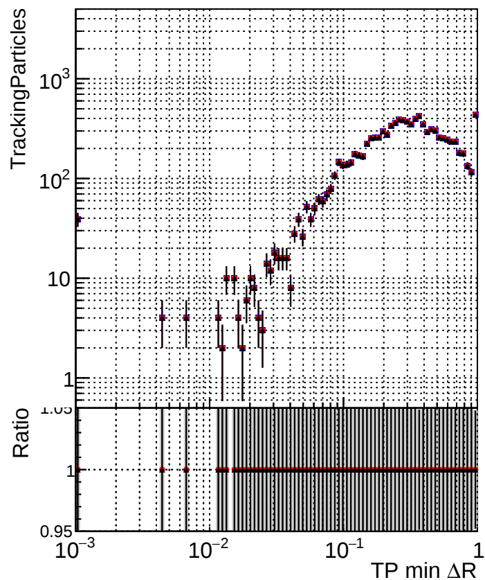
N of simulated tracks vs TP \Delta R (TP, jet) —■— DQM_original_step2_pt1000_eta1p6to2p0 —●— DQM_mkFit_step2_pt1000_eta1p6to2p0 —▲— DQM_pixelCPETemplate_step2_pt1000_eta1p6to2p0
