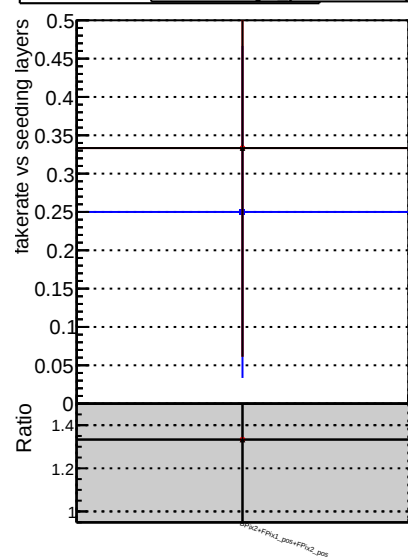
Fake rate vs. DOM original step2 pt1000 eta1p6to2p0 mkr-it step2 pt1000 eta1p6to2p0 DOM pixelCPE template step2 pt1000 eta1p6to2p0
