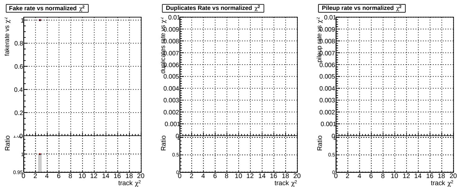
Fake rate vs. DOM original step2 pt1000 eta1p6to2p0 mkr-it step2 pt1000 eta1p6to2p0 DOM pixelCPE template step2 pt1000 eta1p6to2p0
