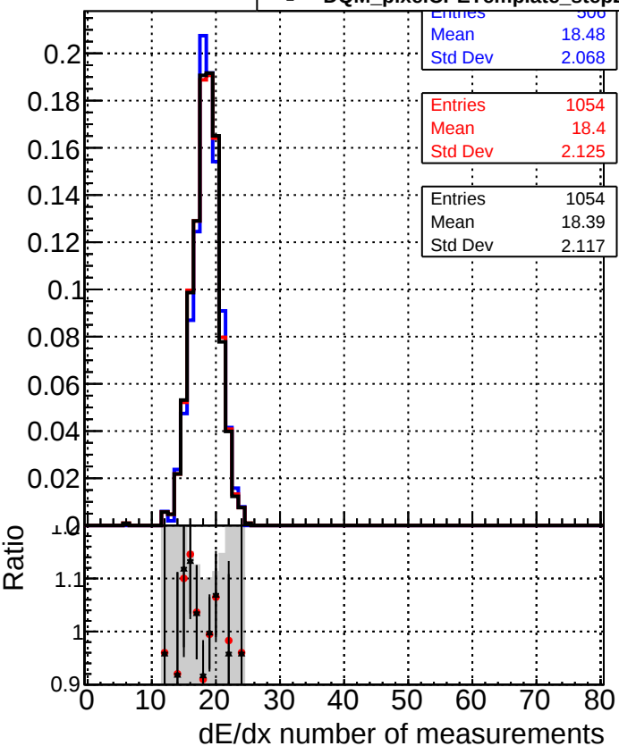
—■— DQM_original_step2_pt1000_eta1p6to2p0 —●— DQM_mkFit_step2_pt1000_eta1p6to2p0 —+— DQM_pixelCPETemplate_step2_pt1000_eta1p6to2p0
