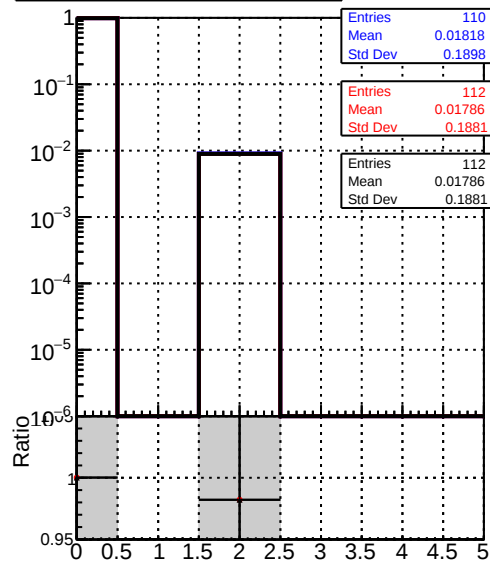
mean hits — DQM_original_step2_pt1000_eta1p6to2p0 — DQM_mkFit_step2_pt1000_eta1p6to2p0 — DQM_pixelCPETemplate_step2_pt1000_eta1p6to2p0
