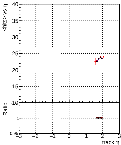
mean hits vs \eta — DQM_original_step2_pt1000_eta1p6to2p0 — DQM_mkFit_step2_pt1000_eta1p6to2p0 — DQM_pixelCPETemplate_step2_pt1000_eta1p6to2p0
