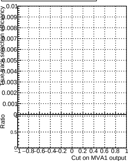
N of associated tracks (recoToSim) vs cut on MVA1
