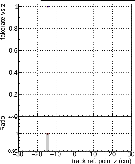
Fake rate vs v DQM_original_step2_pt1000_eta1p4to1p6 DQM_mkFit_step2_pt1000_eta1p4to1p6 DQM_pixelCPETemplate_step2_pt1000_eta1p4to1p6
