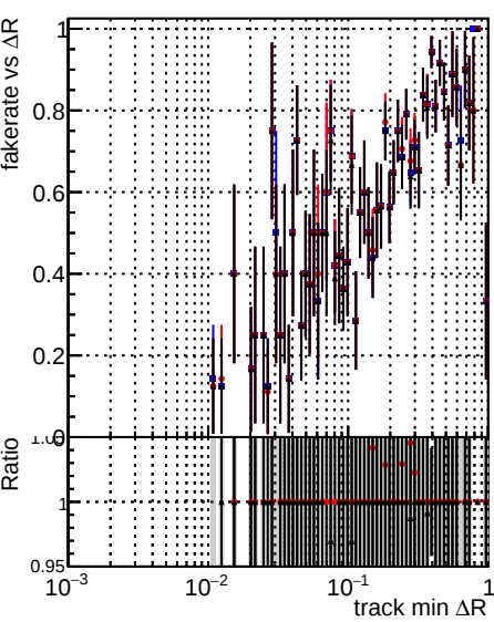
Legend: DQM_original_step2_pt1000_eta1p4to1p6 (blue), DQM_mkFit_step2_pt1000_eta1p4to1p6 (red), DQM_pixelCPETemplate_step2_pt1000_eta1p4to1p6 (black)
