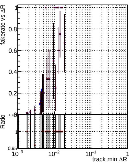
Legend: - \Delta R original step2_pt1000_eta1p4to1p6 (blue line with dots) - \Delta R mkFit step2_pt1000_eta1p4to1p6 (red line with dots) - \Delta R pixelCPETemplate step2_pt1000_eta1p4to1p6 (black line with dots)
