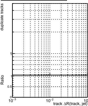
N of associated (recoToSim) loop tracks vs dR(\text{track}, \text{jet})
