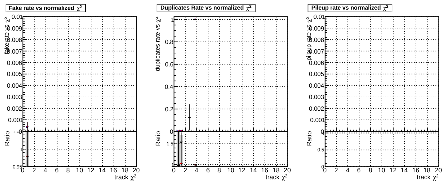
DOM original step2 - pt1000 eta1p4to1p6 DOM mkr-it step2 - pt1000 eta1p4to1p6 DOM pixelCPE template step2 - pt1000 eta1p4to1p6
