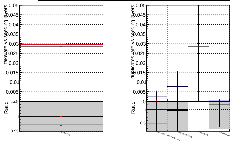
DOM original step2 - pt1000 eta1p4to1p6 DOM mkr-it step2 - pt1000 eta1p4to1p6 DOM pixelCPE template step2 - pt1000 eta1p4to1p6
