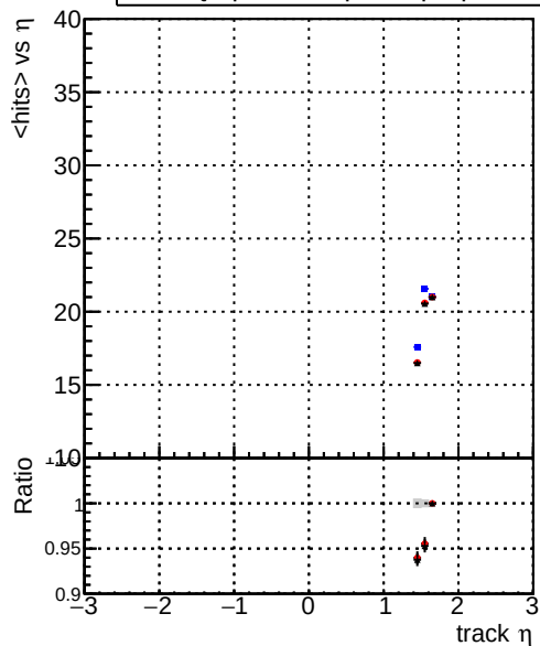
mean hits — DQM_original_step2_pt1000_eta1p4to1p6 — DQM_mkFit_step2_pt1000_eta1p4to1p6 — DQM_pixelCPETemplate_step2_pt1000_eta1p4to1p6
