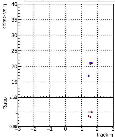
mean hits vs \eta — DQM_original_step2_pt1000_eta1p4to1p6 — DQM_mkFit_step2_pt1000_eta1p4to1p6 — DQM_pixelCPEtemplate_step2_pt1000_eta1p4to1p6
