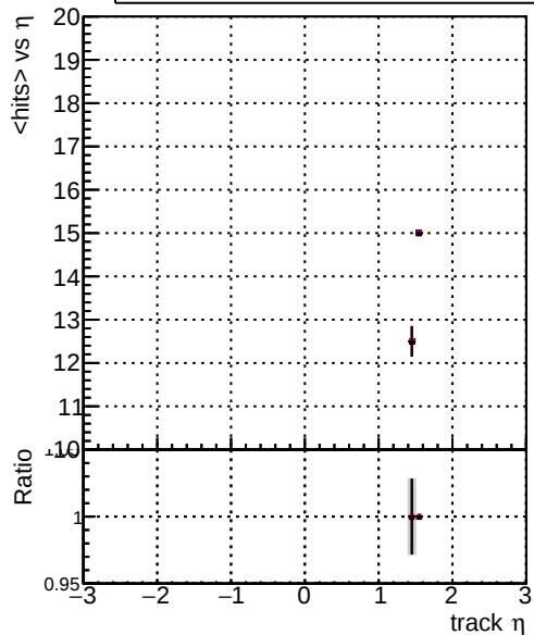
mean hit — DQM_original_step2_pt1000_eta1p4to1p6 — DQM_mkFit_step2_pt1000_eta1p4to1p6 — DQM_pixelCPETemplate_step2_pt1000_eta1p4to1p6
