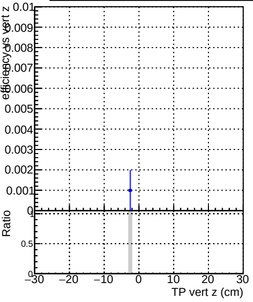
Efficiency vs. TP vert z Legend: DQM_original_step2_pt1000_eta1p4to1p6 DQM_mkFit_step2_pt1000_eta1p4to1p6 DQM_pixelCPETemplate_step2_pt1000_eta1p4to1p6
