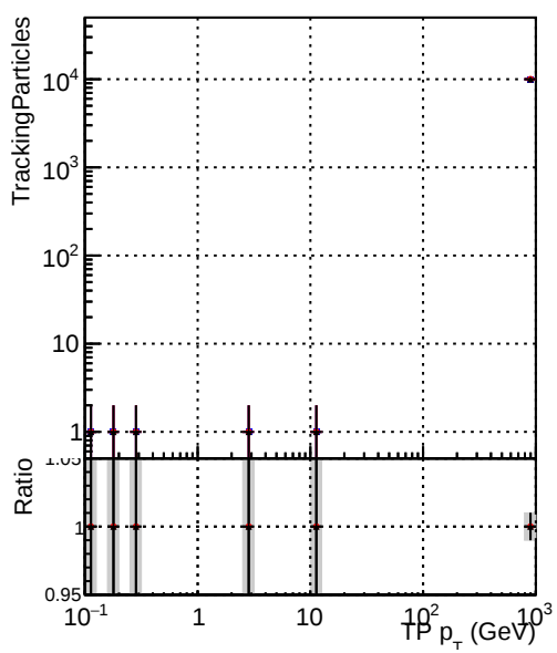
Legend: DQM_original_step2_pt1000_eta1p4to1p6, DQM_mkFit_step2_pt1000_eta1p4to1p6, DQM_pixelCPETemplate_step2_pt1000_eta1p4to1p6
