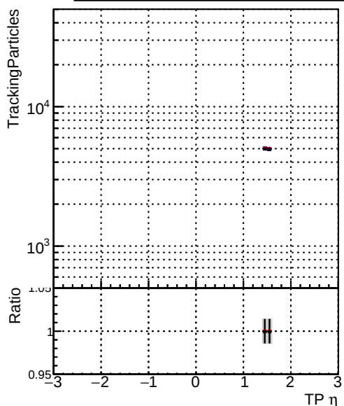
Legend: DQM_original_step2_pt1000_eta1p4to1p6, DQM_mkFit_step2_pt1000_eta1p4to1p6, DQM_pixelCPETemplate_step2_pt1000_eta1p4to1p6
