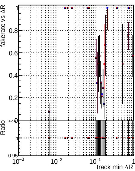
Legend: DQM_original_step2_pt1000_eta1p0to1p4 (blue), DQM_mkFit_step2_pt1000_eta1p0to1p4 (red), DQM_pixelCPETemplate_step2_pt1000_eta1p0to1p4 (black)
