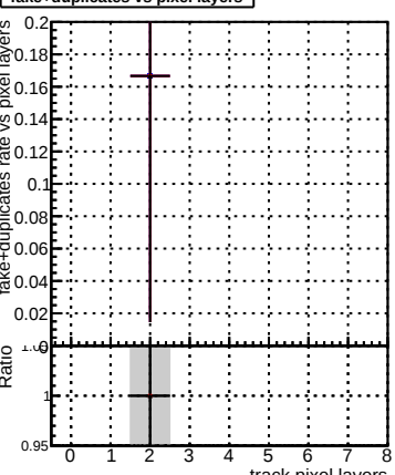
fake+duplicates vs pixel layer
