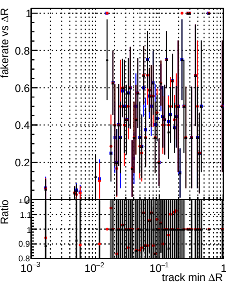
Legend: DQM original step2 pt1000 eta1p0to1p4 (blue), DQM mkFit step2 pt1000 eta1p0to1p4 (red), DQM pixelCPE template step2 pt1000 eta1p0to1p4 (black)
