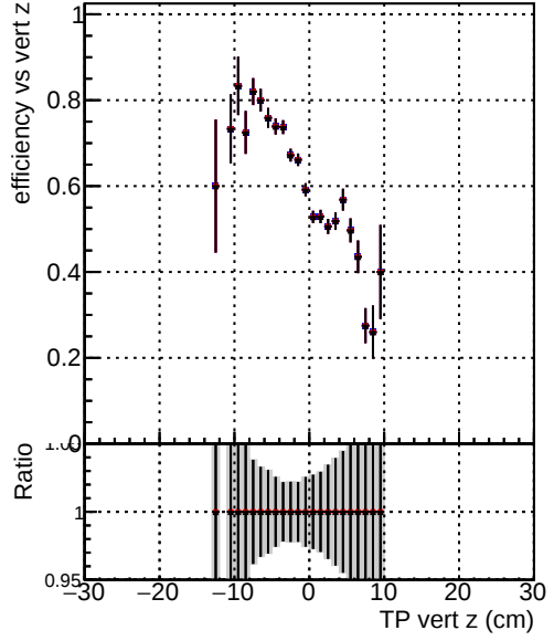
Efficiency vs. sim PV z —•— DQM_original_step2_pt1000_eta1p0to1p4 —•— DQM_mkFit_step2_pt1000_eta1p0to1p4 —•— DQM_pixelCPETemplate_step2_pt1000_eta1p0to1p4
