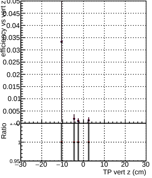
Efficiency vs TP vert z Legend: DQM_original_step2_pt1000_eta1p0to1p4 DQM_mkFit_step2_pt1000_eta1p0to1p4 DQM_pixelCPETemplate_step2_pt1000_eta1p0to1p4
