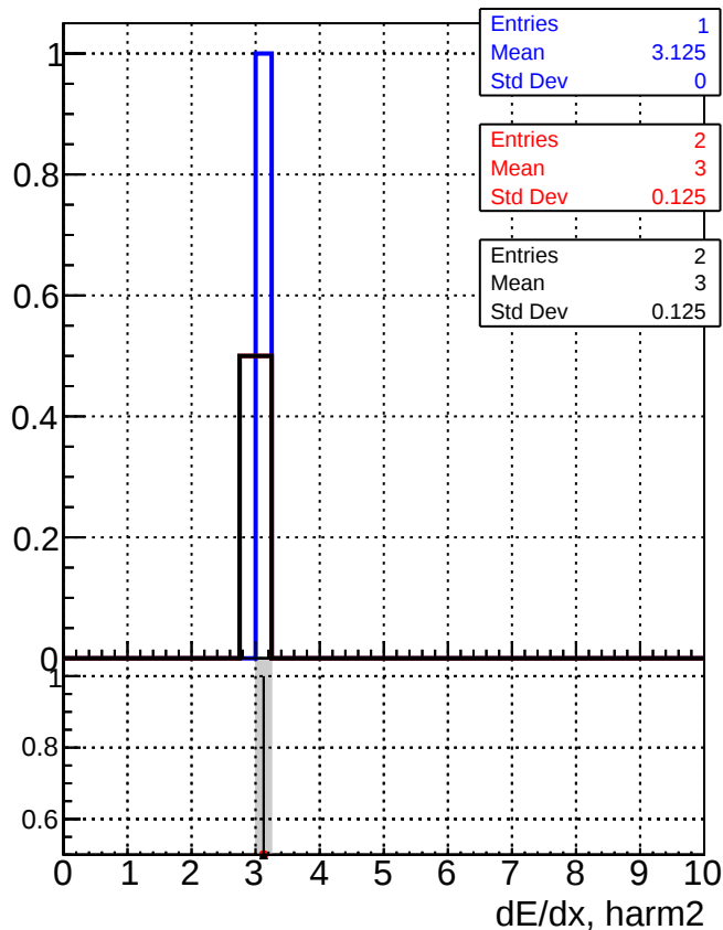
—■— DQM_original_step2_pt1000_eta1p0to1p4 —●— DQM_mkFit_step2_pt1000_eta1p0to1p4 —▲— DQM_pixelCPETemplate_step2_pt1000_eta1p0to1p4
