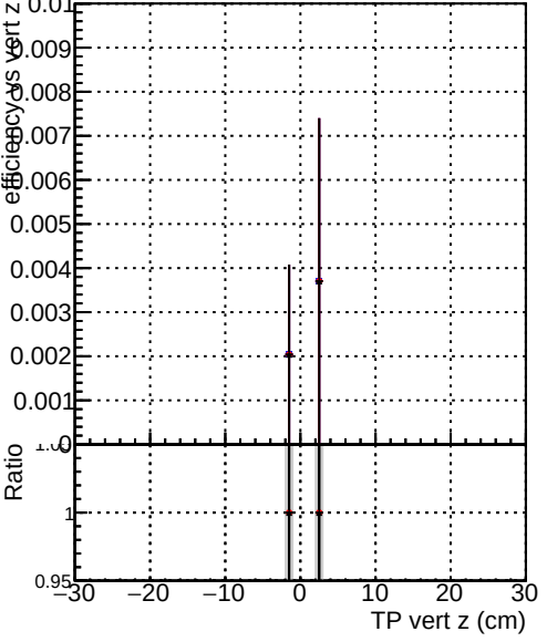
Efficiency vs vert z Legend: DQM_original_step2_pt1000_eta1p0to1p4 DQM_mkFit_step2_pt1000_eta1p0to1p4 DQM_pixelCPETemplate_step2_pt1000_eta1p0to1p4
