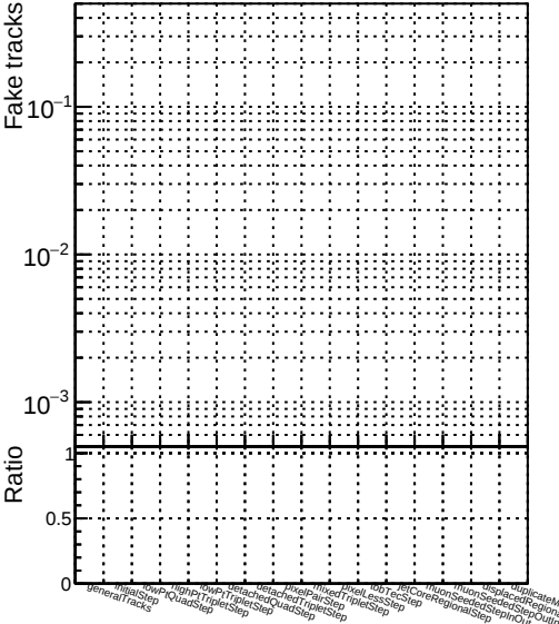
Number —●— DQM_mkFit_step2_pt1000_eta1p0to1p4 —★— DQM_pixelCPETemplate_step2_pt1000_eta1p0to1p4
