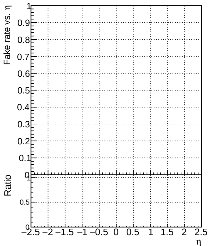
\Lambda tracking fake rate vs \eta
