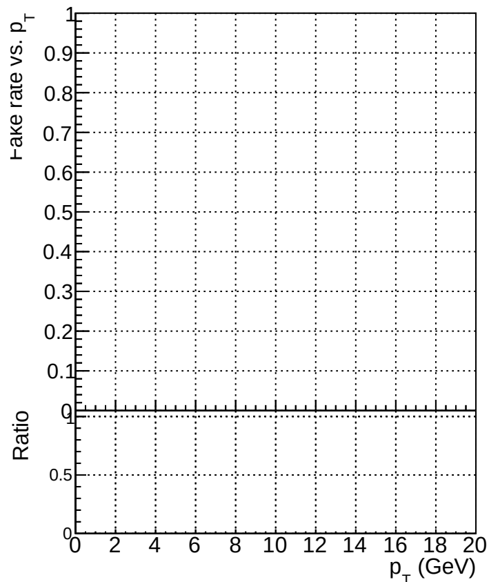
\Lambda tracking fake rate vs p_T
