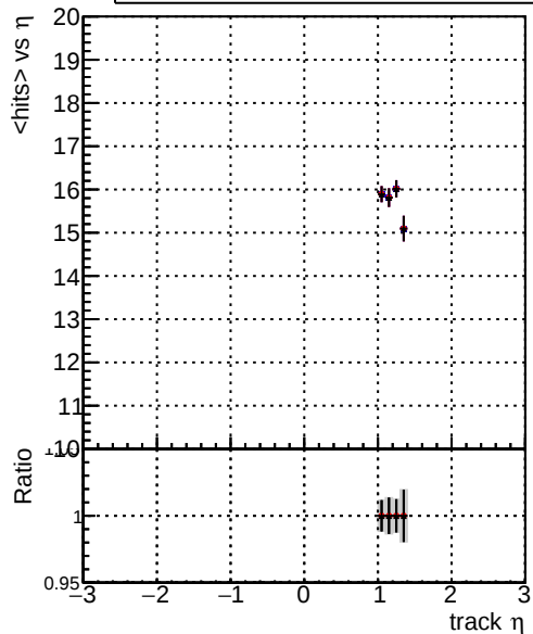
mean hits — DQM_original_step2_pt1000_eta1p0to1p4 — DQM_mkFit_step2_pt1000_eta1p0to1p4 — DQM_pixelCPETemplate_step2_pt1000_eta1p0to1p4
