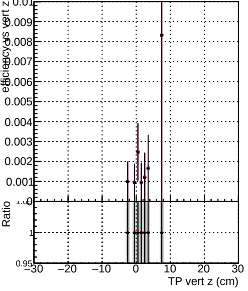
Efficiency vs TP vert z (cm) and fake+duplicates vs track ref. point z (cm) Legend: DQM_original_step2_pt1000_eta1p0to1p4 DQM_mkFit_step2_pt1000_eta1p0to1p4 DQM_pixelCPETemplate_step2_pt1000_eta1p0to1p4
