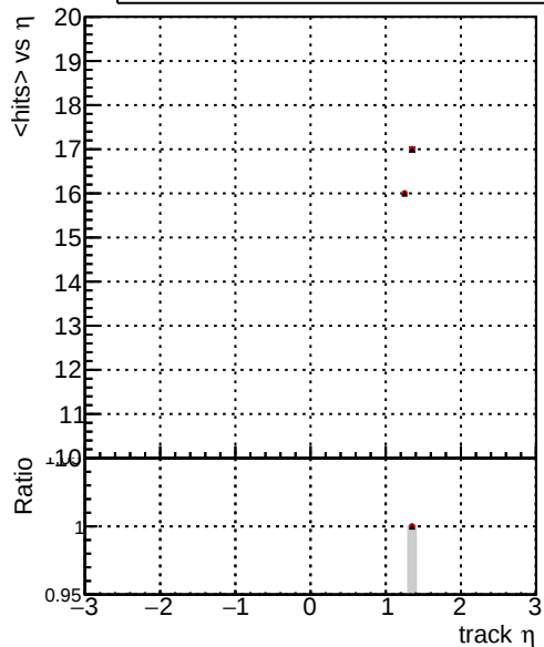
— DQM_original_step2_pt1000_eta1p0to1p4 — DQM_mkFit_step2_pt1000_eta1p0to1p4 — DQM_pixelCPETemplate_step2_pt1000_eta1p0to1p4
