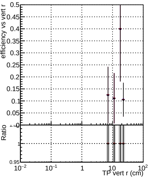
Efficiency vs TP vert r (cm) Legend: DQM_original_step2_pt1000_eta0p4to1p0 DQM_mkFit_step2_pt1000_eta0p4to1p0 DQM_pixelCPETemplate_step2_pt1000_eta0p4to1p0
