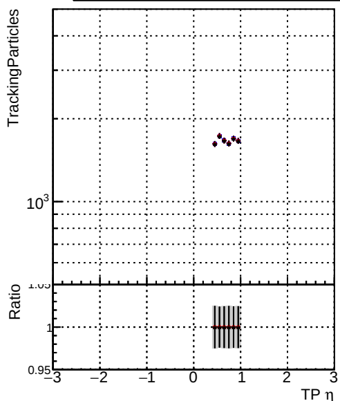
N of simulated tracks vs TP eta N of associated tracks (simToReco) vs TP eta Legend: DQM_original_step2_pt1000_eta0p4to1p0 DQM_mkFit_step2_pt1000_eta0p4to1p0 DQM_pixelCPETemplate_step2_pt1000_eta0p4to1p0
