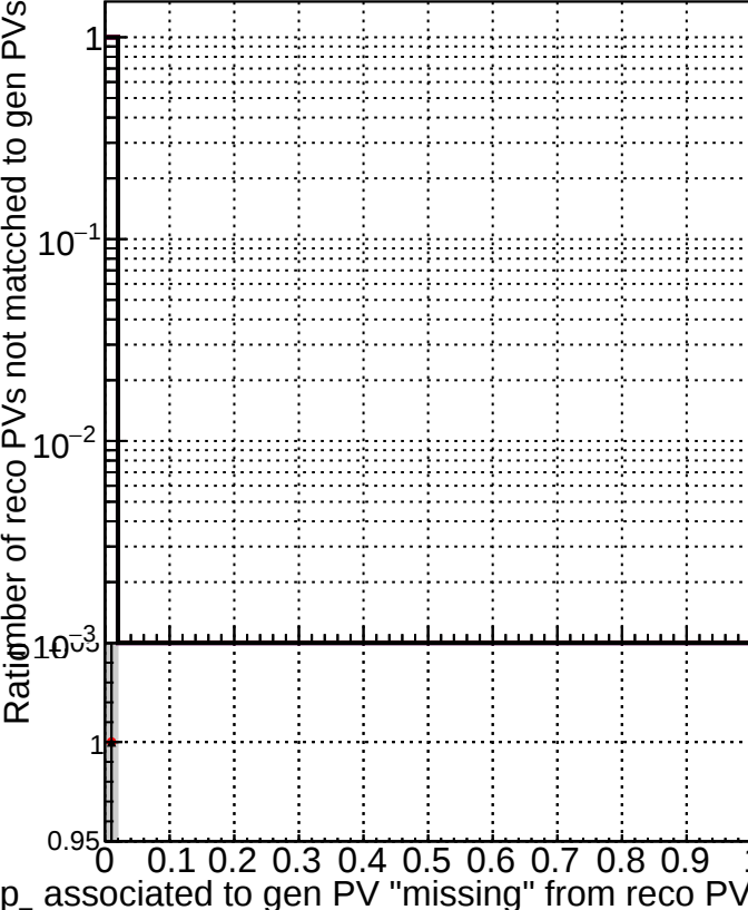
RECOPVASSOCZGENPVNOTmatched_MISSING
