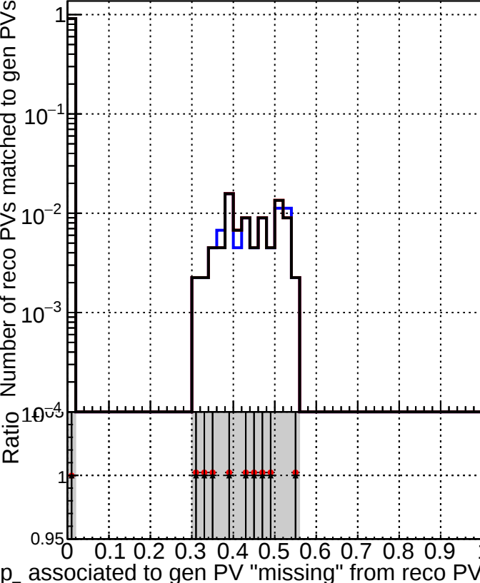
RecoPVAssoc2GenPVmatched_missing
