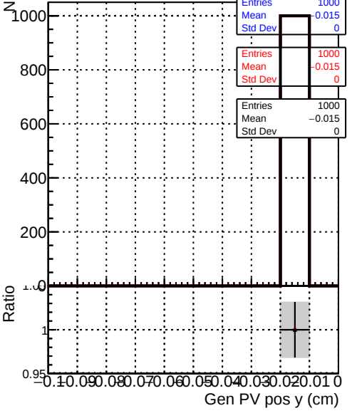
GeneratedAllV_Y Legend: DQM_original_step2_pt1000_eta0p4to1p0 (blue line) DQM_mkFit_step2_pt1000_eta0p4to1p0 (red line) DQM_pixelCPETemplate_step2_pt1000_eta0p4to1p0 (black line)
