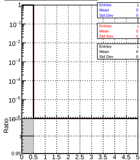
mean hit DQM_original_step2_pt1000_eta0p4to1p0 DQM_mkFit_step2_pt1000_eta0p4to1p0 DQM_pixelCPETemplate_step2_pt1000_eta0p4to1p0
